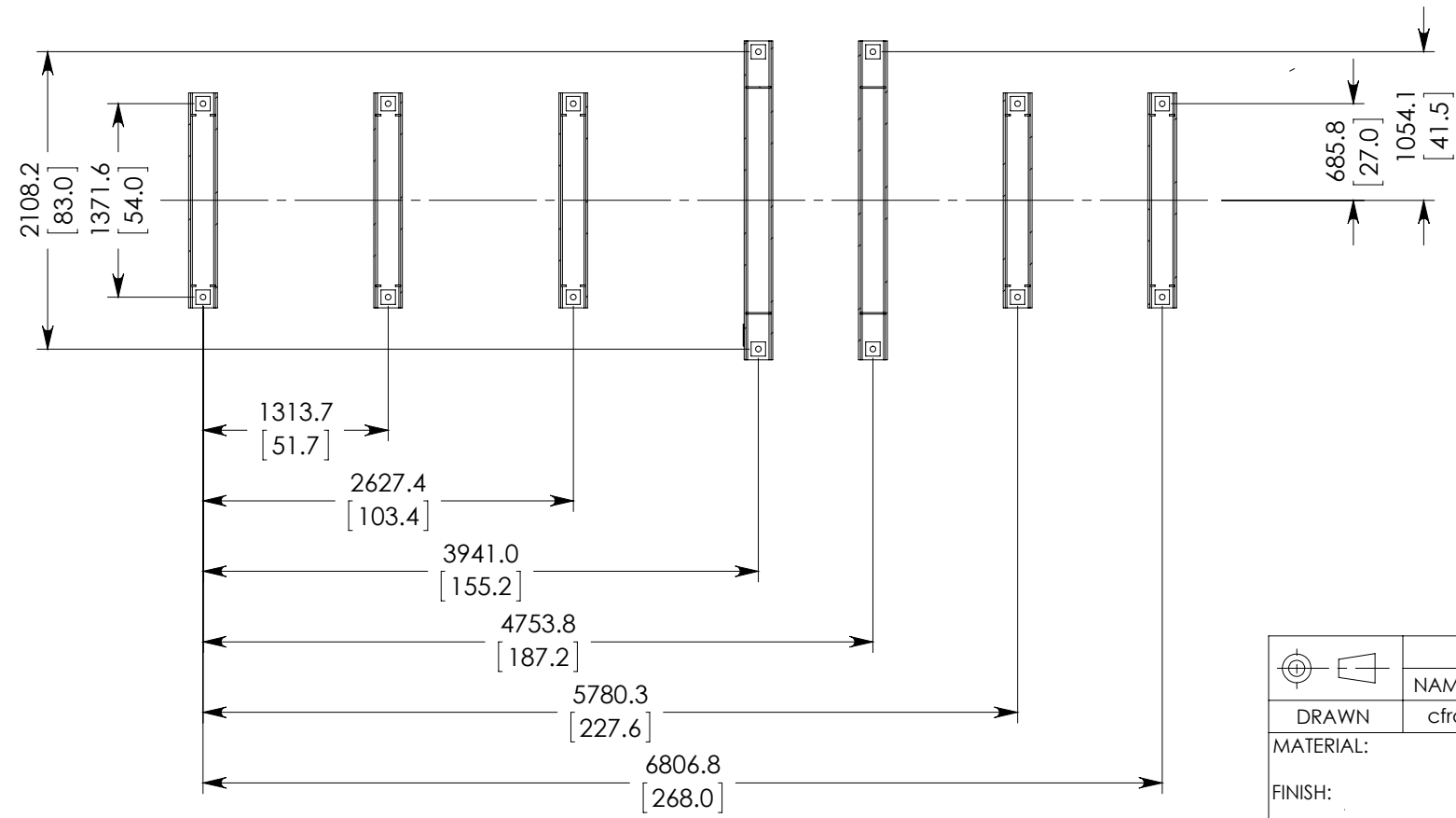
BASE MOUNTING HOLES
